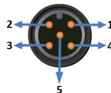
M12 5 IN MALE CONN.
